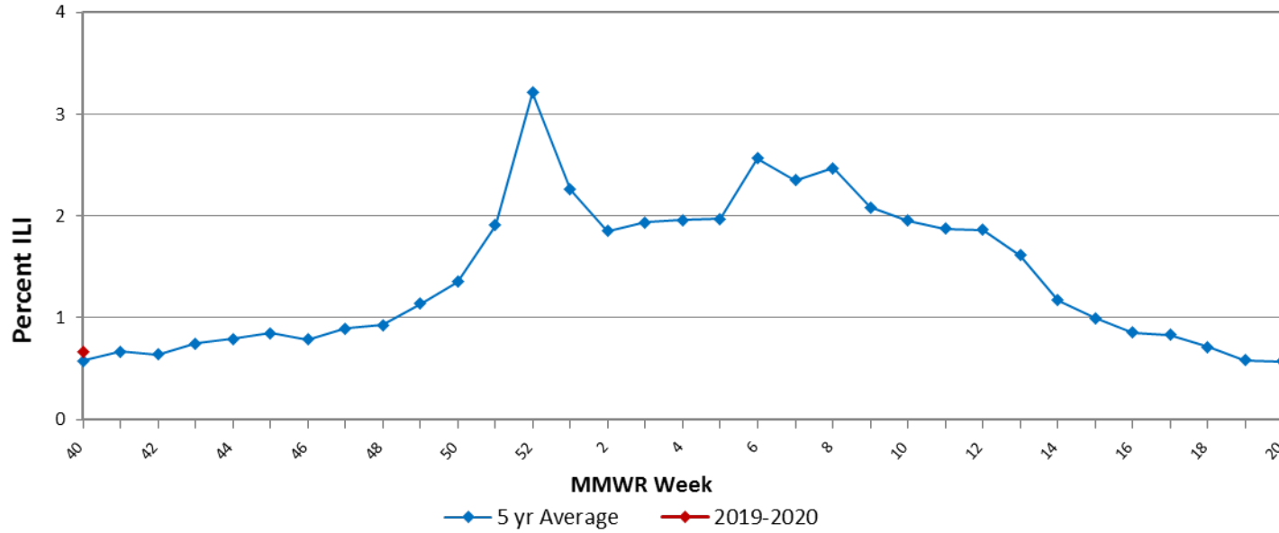
Ohio Outpatient Influenza-like Illness Network (ILINet) with 5 Year Baseline Average; 2019-2020
