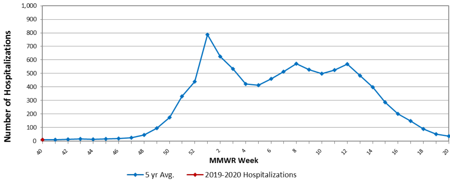
Ohio Confirmed Influenza-associated Hospitalizations by MMWR Week; 2019-2020 Season (n=8)
